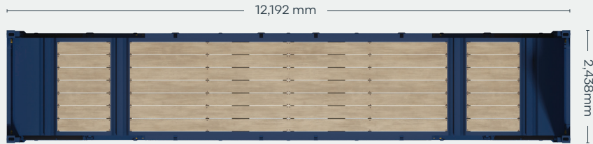
FLATRACK TOP
